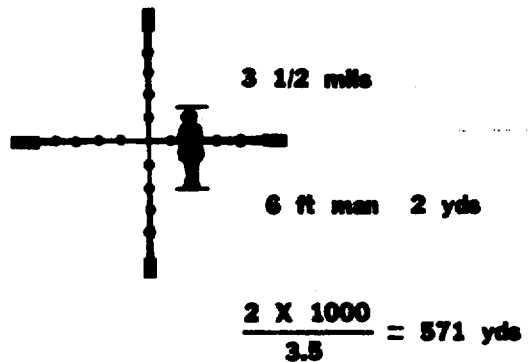
Figure 2-10. Mil Dot Reticle.
